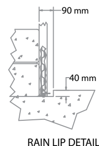
FIGURE 4 UNIVERSAL MOUNT GUIDES
