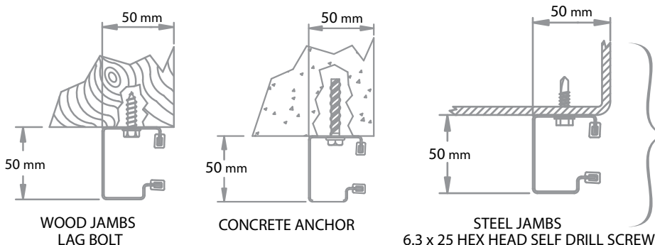
FIGURE 4 UNIVERSAL MOUNT GUIDES
